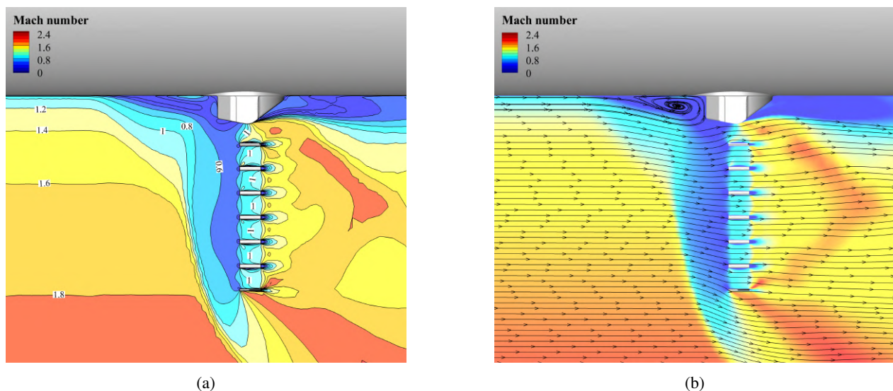
Figure 9: Gridfin flowfield for Mach 2 baseline case showing (a) Mach contours and (b) flow streamtraces
