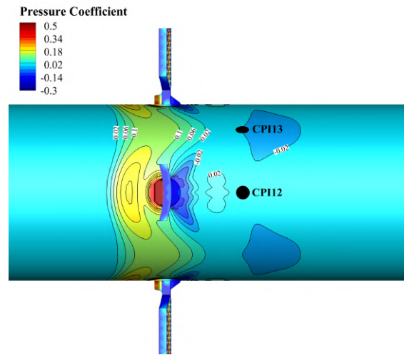
Figure 8: Surface pressure contours at sensor locations 12 and 13 for Mach 2 baseline case
