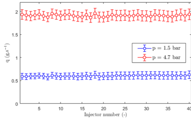
Figure 10: Mean flow rate measured in each injector once installed on the compressor test rig for two different levels of supply pressure with continuous actuation, error bars are measurement errors of the flowmeter
