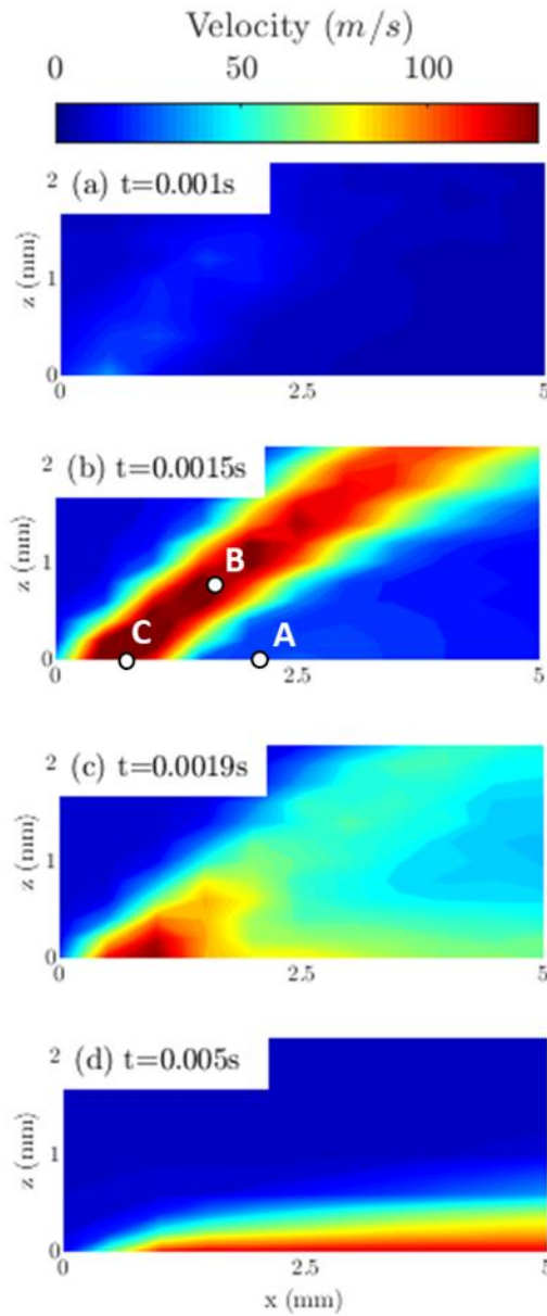
Figure 7: Mean phase - locked maps of velocity magnitude measured in the longitudinal (x,z) plan extracted at different time steps ( f = 100 Hz, p = 2.5 bar, \alpha = 0.4 )
