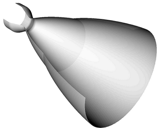
Fig. 1. Dual-bell nozzle
