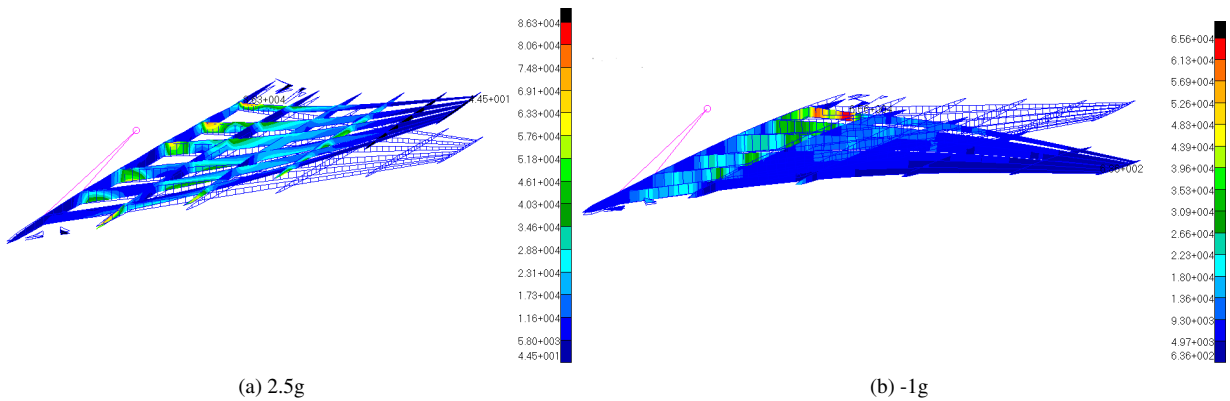
Figure 5: Wing deflection at 2.5g and -1g at Mach 5, coloured by stress level.
