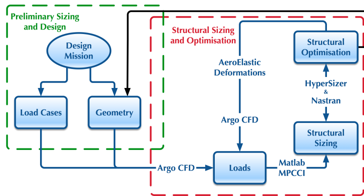
Figure 2: The Sizing Process Used for the A2 Structure
