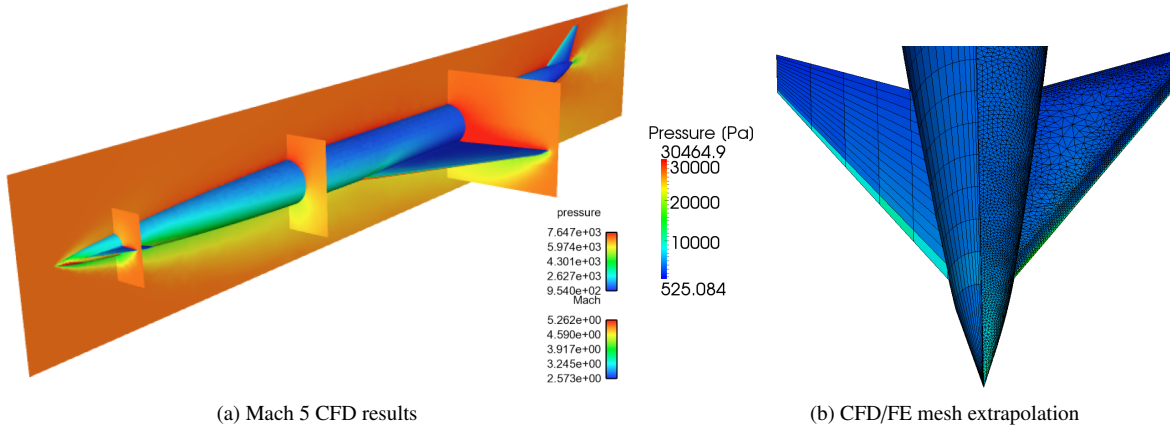
Figure 3: CFD results and CFD/FE mesh translation.
