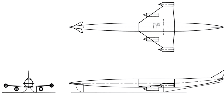
Figure 1: The LAPCAT A2 configuration for a Mach 5 TBCC vehicle based on hydrogen 1
