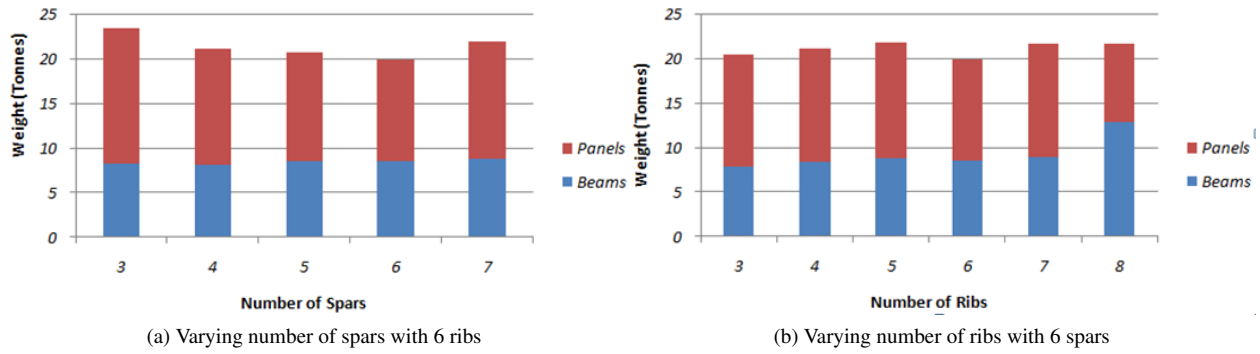
Figure 4: Wing weight for varying numbers of ribs and spars.
