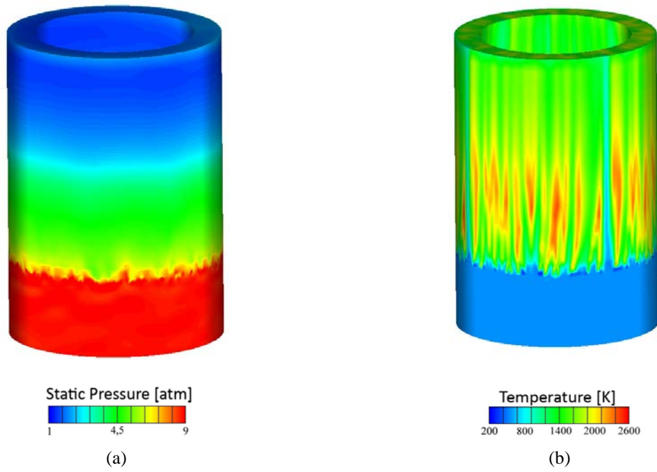
Figure 5: Instantaneous distributions of (a) static pressure and (b) temperature near the outer wall of the CDC operating in the stabilized deflagration mode in Run 3
