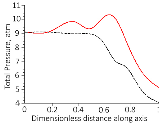
Figure 9: Estimated distribution of the total pressure averaged over the cross section in the annular combustion chamber with detonation (solid red curve, Run1) and deflagration (dashed black curve, Run 3)
