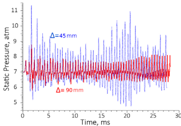
Figure 8: Predicted time histories of static pressure in the upstream isolators of different width
