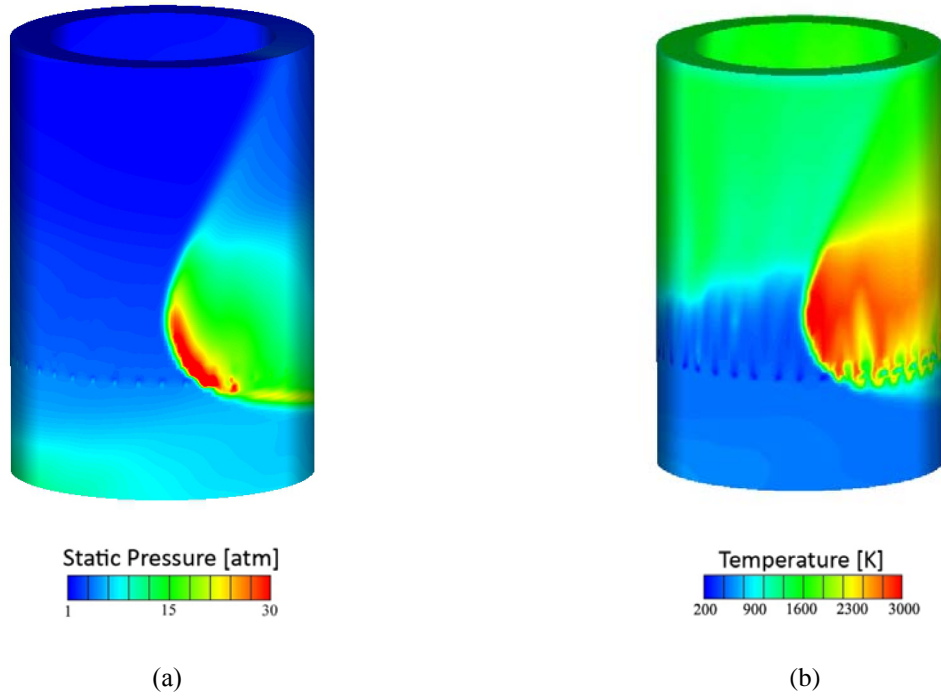
Figure 4: Instantaneous distributions of (a) static pressure and (b) temperature near the outer wall of the CDC operating in the continuous detonation mode in Run 1. Detonation propagates from right to left
