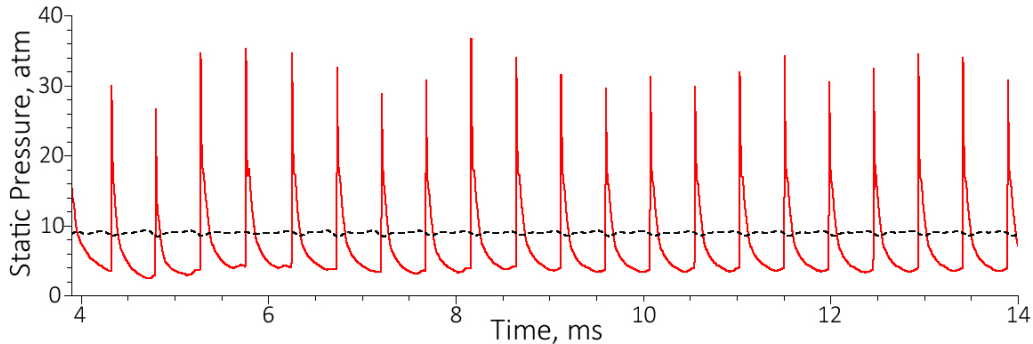
Figure 7: Predicted time histories of static pressure in the middle of the CDC (solid red curve) and in the upstream isolator with \Delta = 90 mm (dashed curve)
