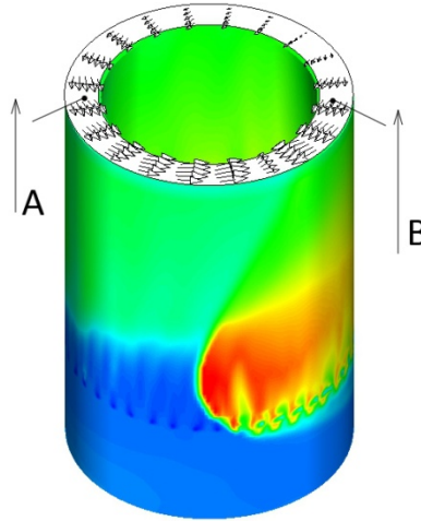
Figure 10: Predicted flow pattern at the CDC exit in Run 1. The lengths of the vectors A and B in the corresponding points represent the scale for the longitudinal velocity component (A: 1470 m/s; B: 1610 m/s). Transverse velocity components have the same scale
