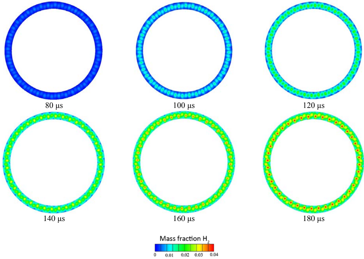
Figure 3: Instantaneous distributions of hydrogen mass fraction in the CDC cross section at the stage of chamber filling with fuel components before detonation initiation in Run 1
