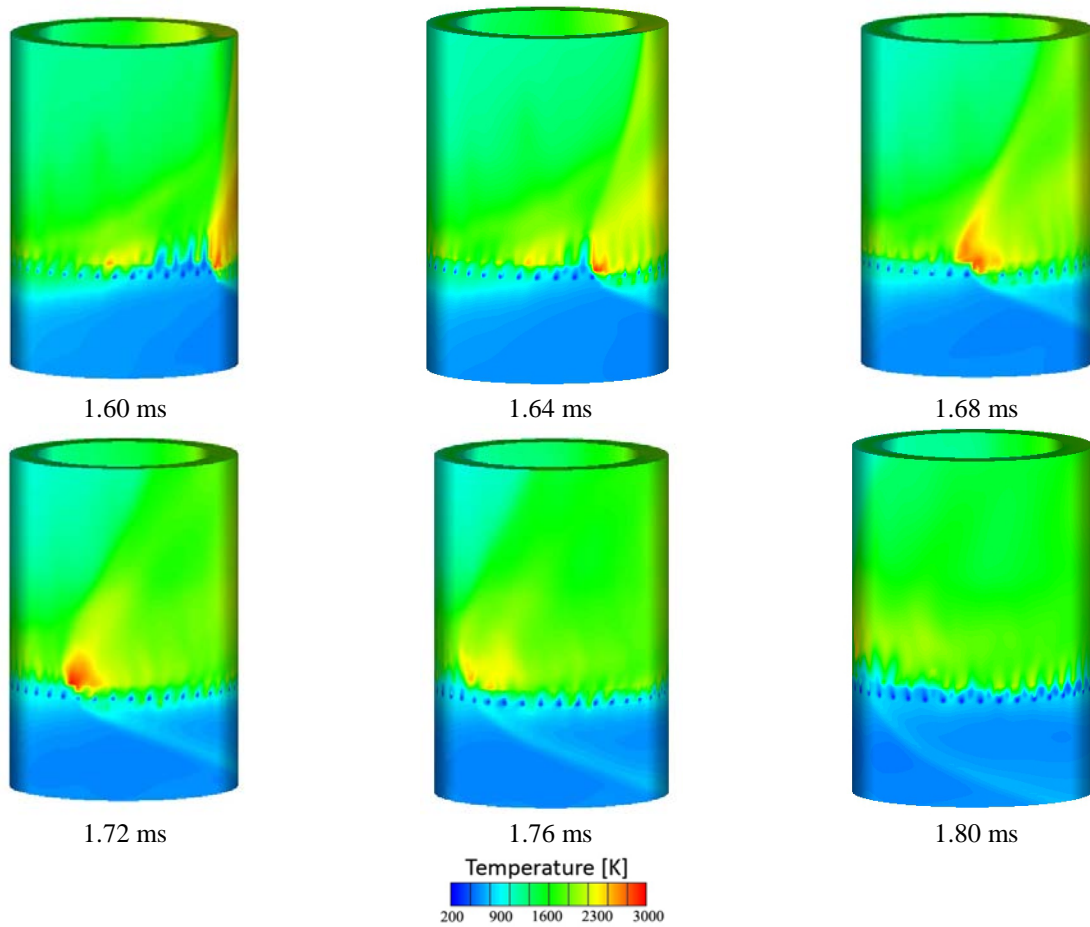
Figure 6: Transition from detonation to stabilized deflagration mode in Run 4
