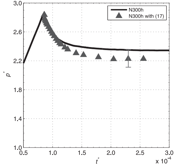
Figure 11: Experimental and analytical pressure drop with Equation (17) of the N300h experiment.
