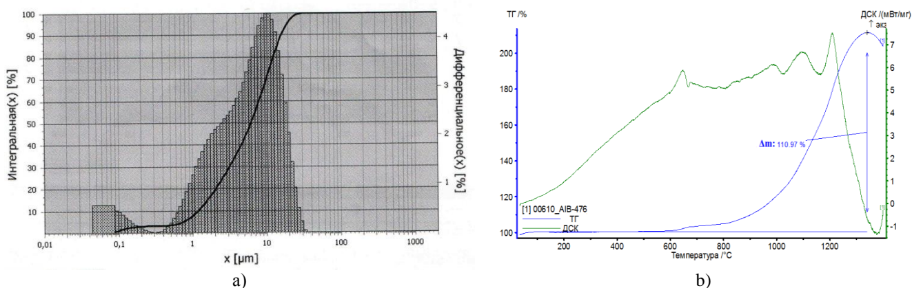
Figure 2. Particle size distribution (a) and DTA analysis data (b) for \text{AlB}_2 powder produced by means of SH synthesis
