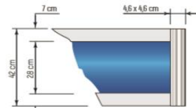
Fascia details
